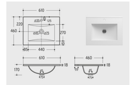
d4 60x46cm Ceramic Basin
