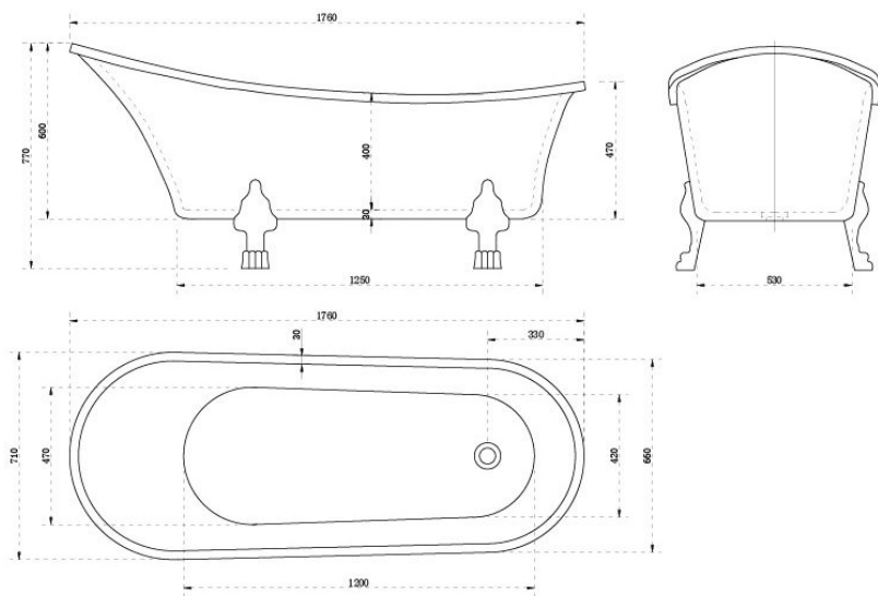
d5 1760 x 710 Freestanding Slipper Bath
