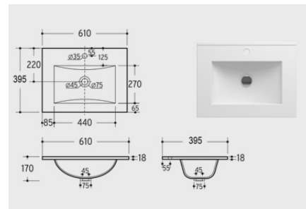
d4 60x40cm Ceramic Basin
