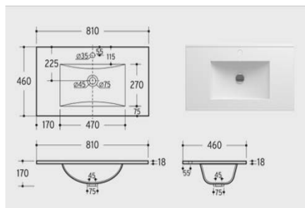
d4 80x46cm Ceramic Basin
