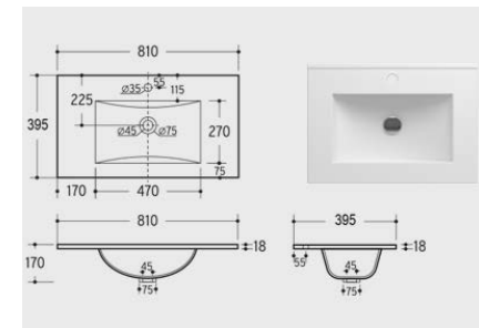
d4 80x40cm Ceramic Basin
