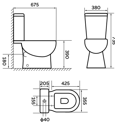
d5 Cistern with Dual Flush Fittings
