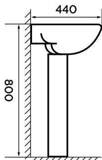
d5 Basin One Tap Hole
