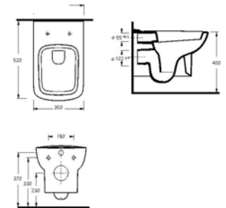
d4 Wall Hung CODE: d4-WH-SQ
