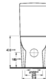
d4 Square Short Projection Toilet Pan
