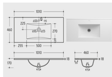
d4 100x46cm Ceramic Basin
