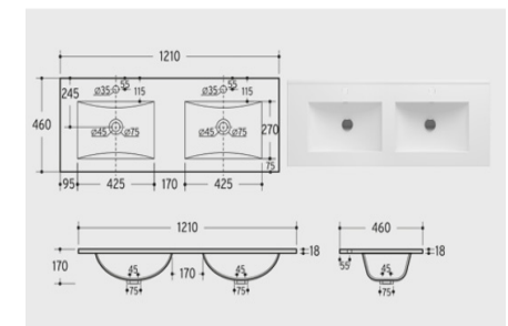
d4 120x46cm Double Ceramic Basin
