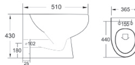
d6 Back to Wall
