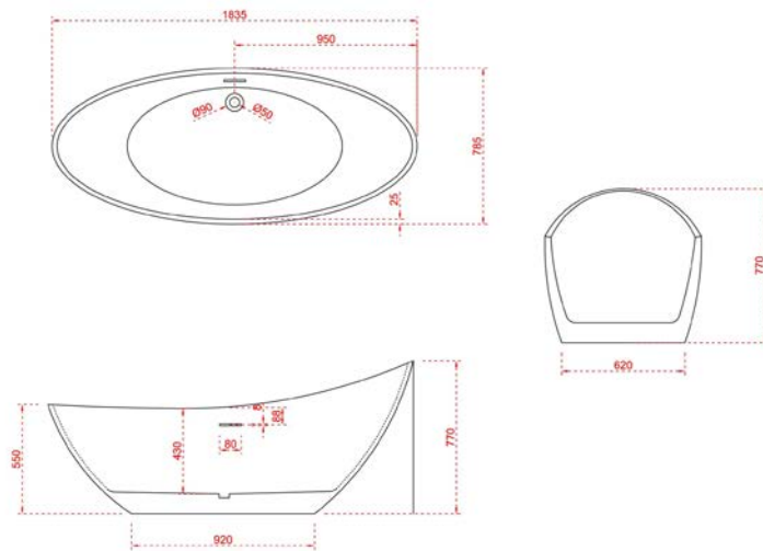
d9 1835 x 785 Freestanding Bath
