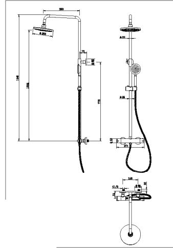
Round Style Thermostatic Shower Valve CODE: d4-RD-SV
