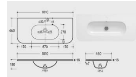
d8 100x46cm Mineral Plus Basin
