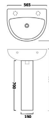
d6 Ped- Basin
