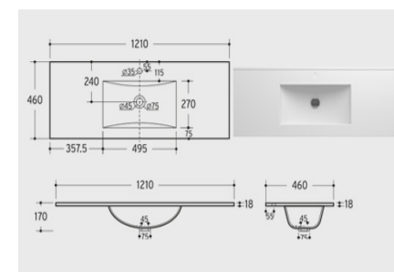
d4 120x46cm Ceramic Basin
