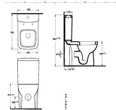
d4 Close Couple Rimless CODE: d4-PAN-SQ CODE: d4-CIS-SQ
