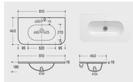
d8 80x46cm Mineral Plus Basin
