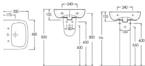
d2 Round 1 Tap Hole Basin 450mm & Semi-Pedestal CODE: d2-BAS-45-35
