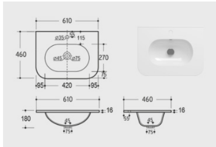
d8 60x46cm Mineral Plus Basin
