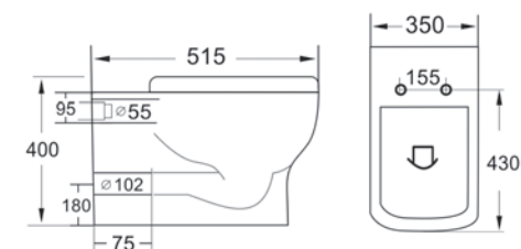
d6 Back to Wall Pan
