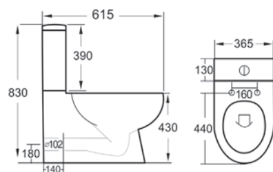
d6 Close Couple Rimless
